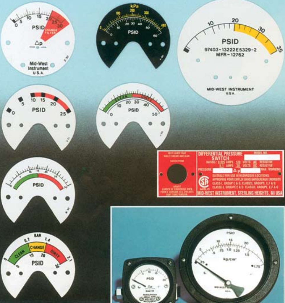
Gauge Dials Can Include Logo, Custom Scales or Units
